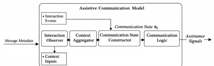
Figure 2: Functional Architecture of the Assistive Communication Model
