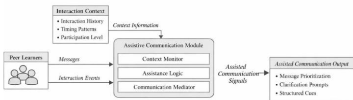
Figure 1: System Architecture of the Assistive Intelligent Communication Framework
